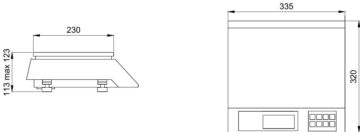
Dimensions (mm)
